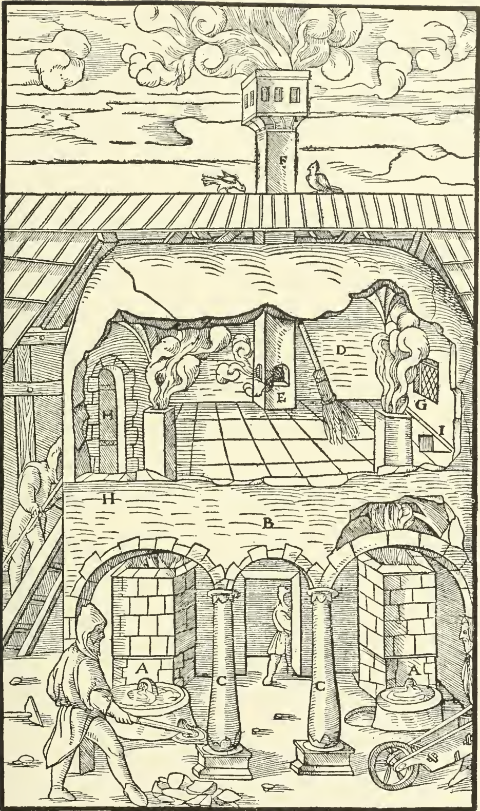
A—FURNACES. B—VAULTED ROOF. C—COLUMNS. D—DUST-CHAMBER. E—OPENING. F—CHIMNEY. G—WINDOW. H—DOOR. I—CHUTE.
